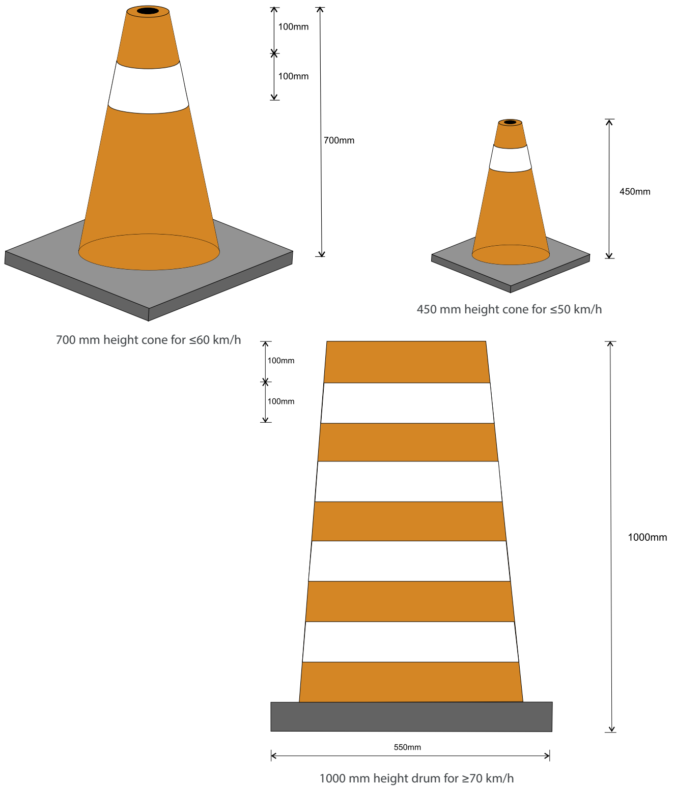
Figure 6: Delineation devices
