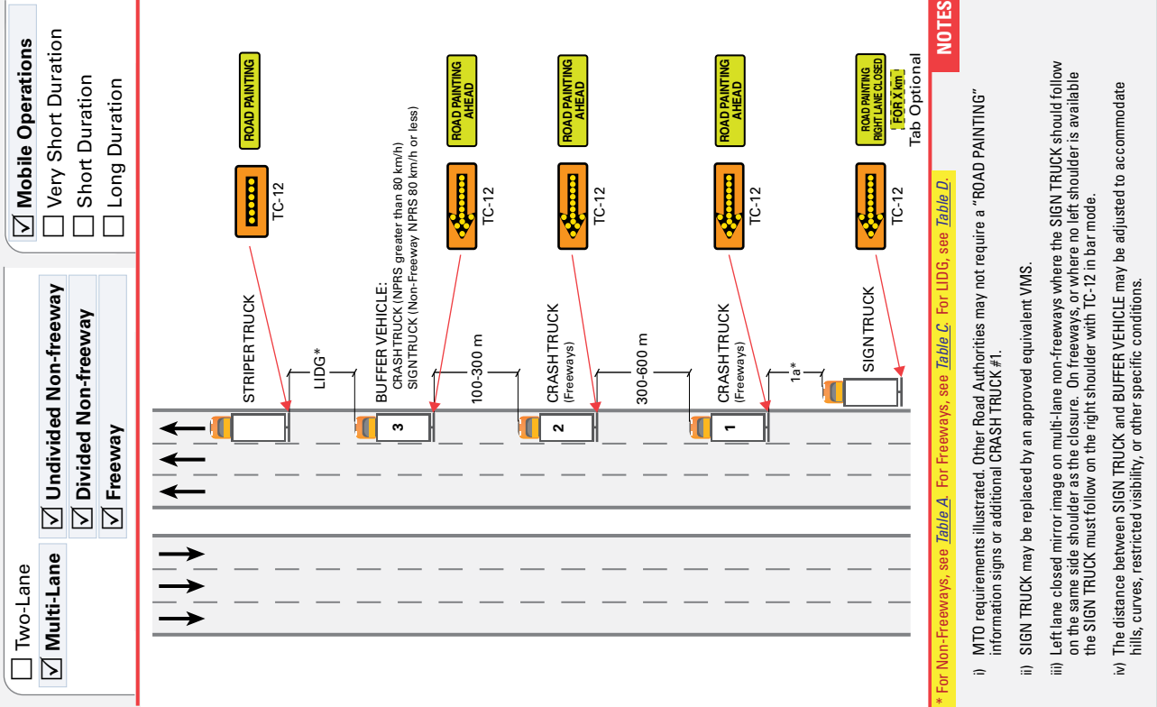
Figure TL-68 Zone Painting: Right or Left Lane Closed (non-coning paint)
