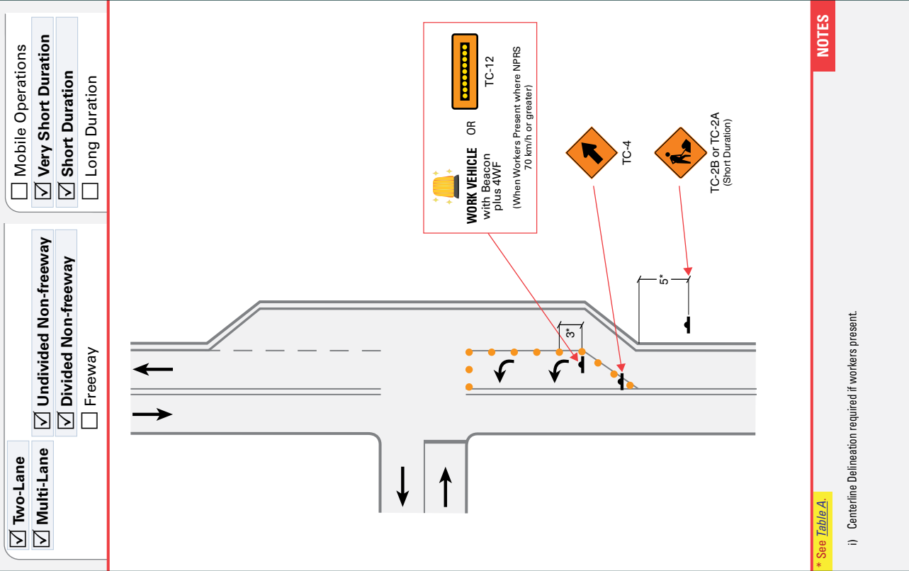
Figure TL-69 Zone Painting: Intersection Turn Arrows
