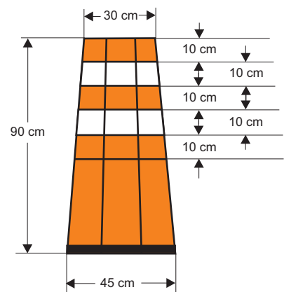
FLEXIBLE DRUMS
