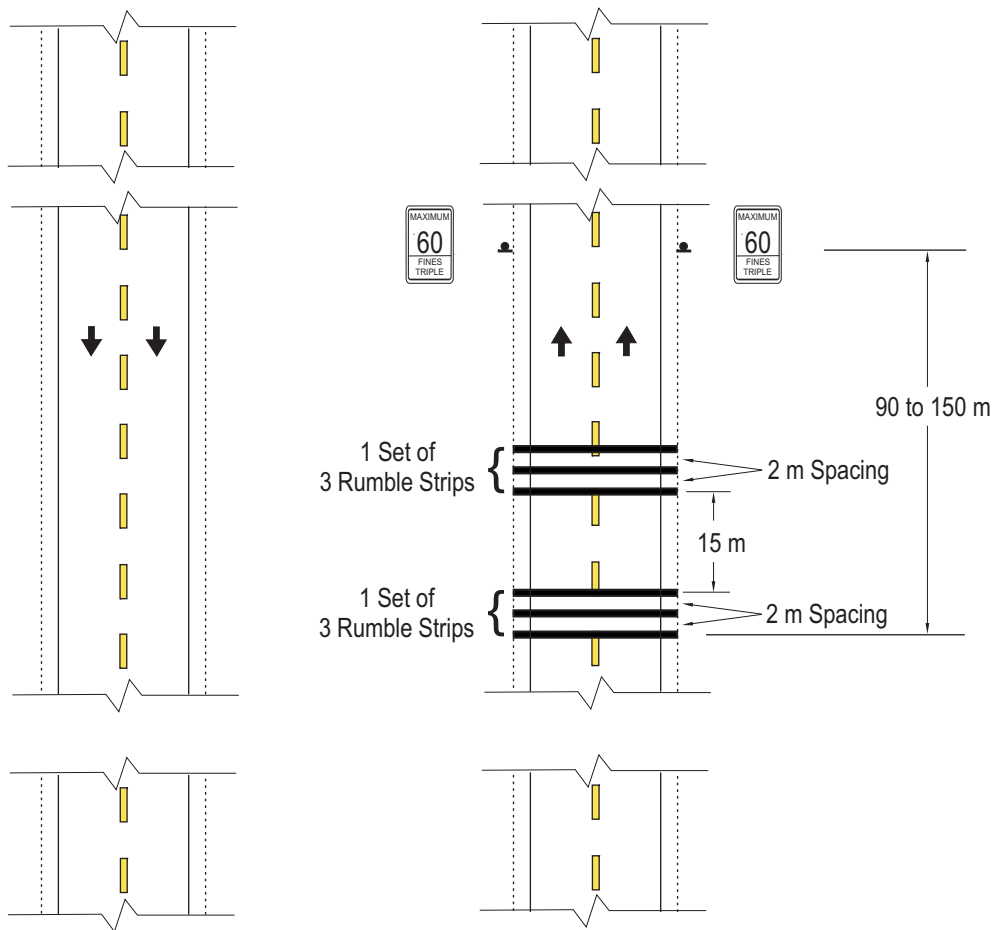
Typical 4 Lane
