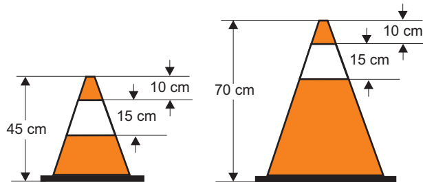
TRAFFIC CONES
