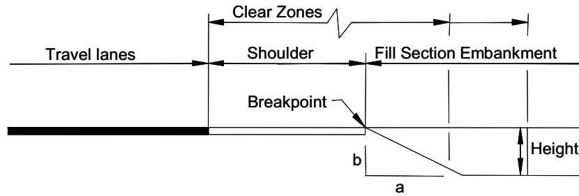
FIGURE H3.5 Warrants for Sideslopes with AADT \geq 400 vpd
